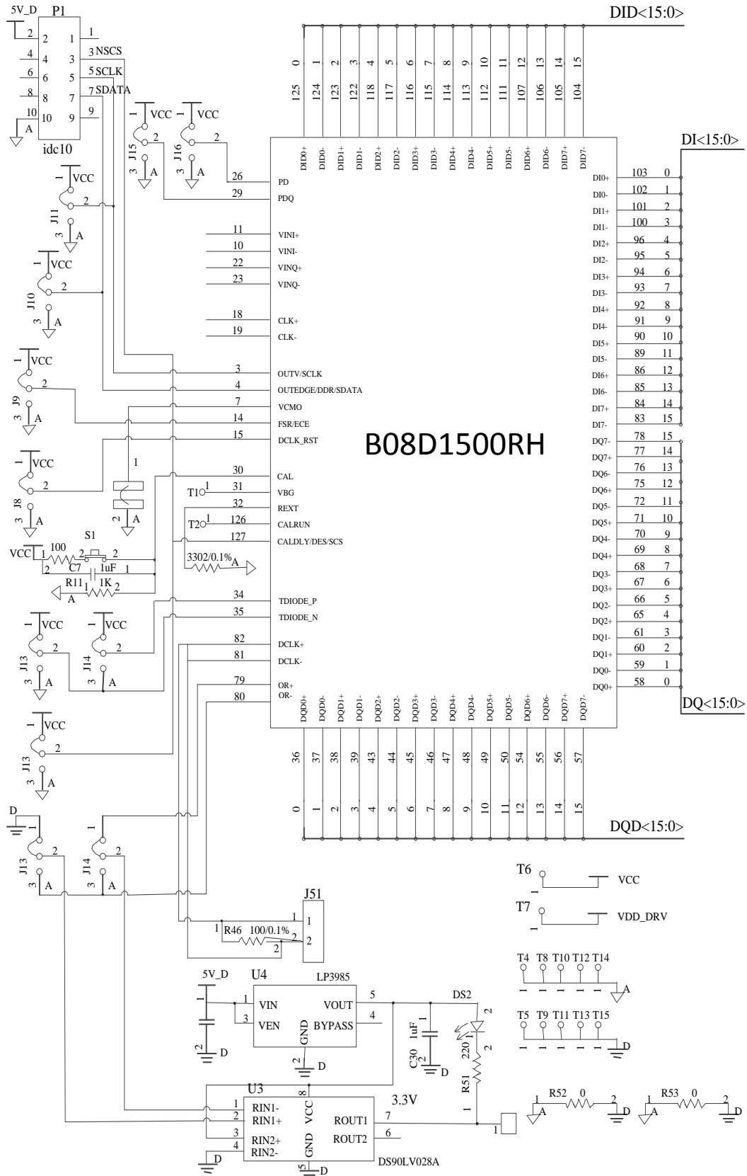
Figure17. The typically application and the peripheral circuit (a)
