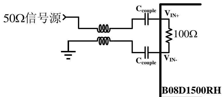
Figure14. Single-Ended to Differential Signal Conversion Using a Balun
