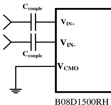
Figure12. Differential Input Drive
