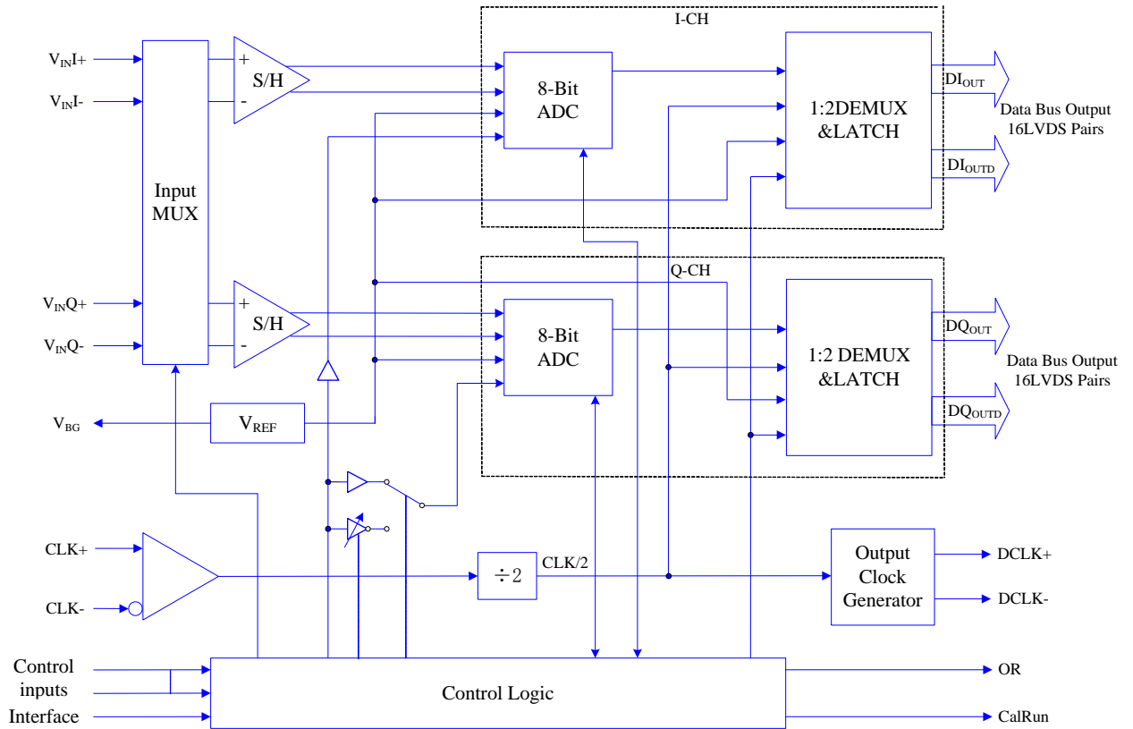
Figure1. Block Diagram
