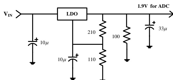
Figure16. Non-Spiking Power Supply
