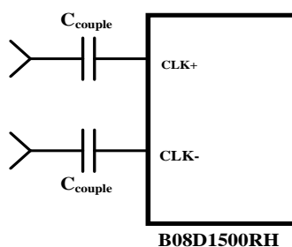
Figure15. Differential (LVDS) Input Clock Connection
