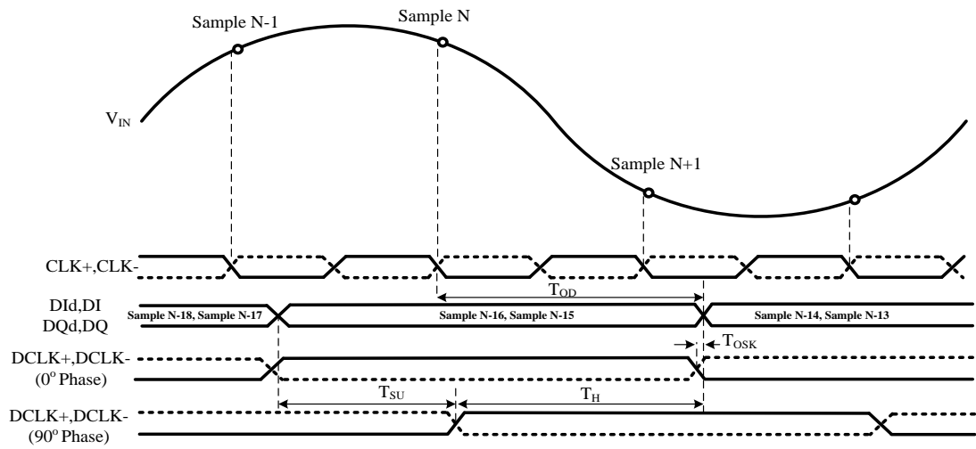
Figure5. B08D1500RH Timing — DDR Clocking
