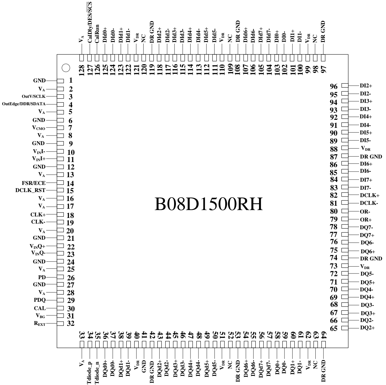
Figure2. Pin configuration
